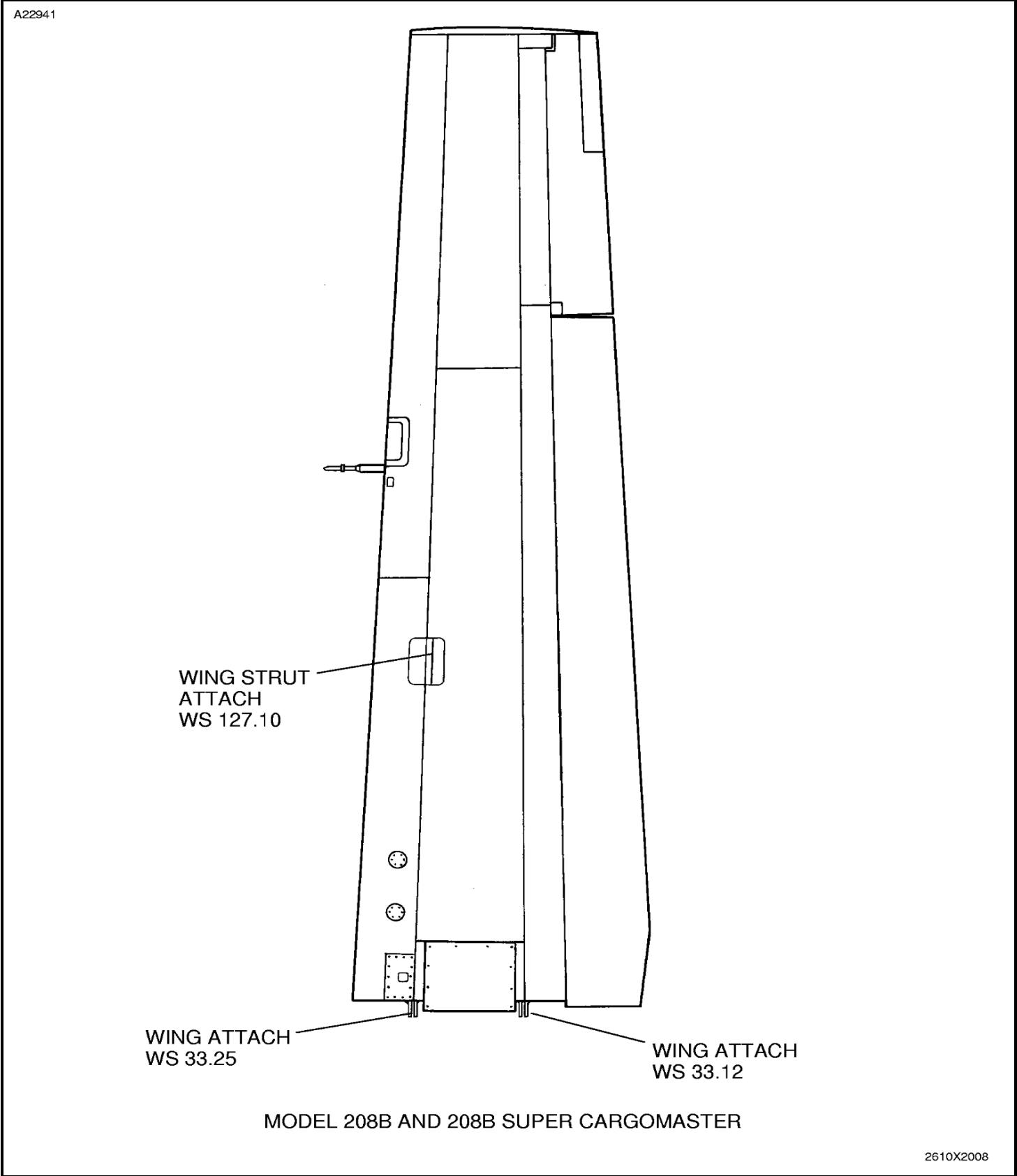
Figure 1 : Sheet 3 : Major Structural Members Locations
