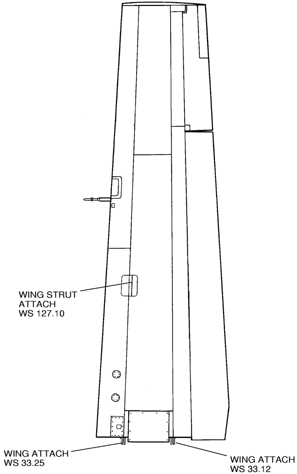
Figure 1 : Sheet 2 : Major Structural Members Locations
